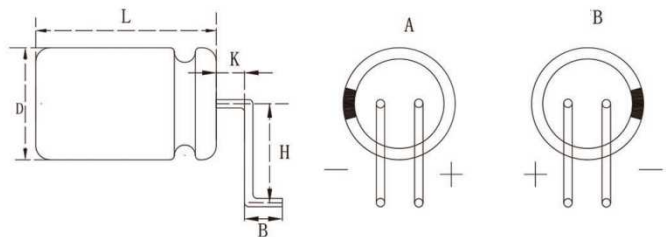
Lead wire cutting and forming H diagram (forming double bend 90° )
