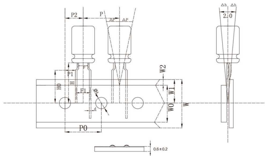
BRAIDED TAPE EXTERNAL DIMENSIONS DIAGRAM B
