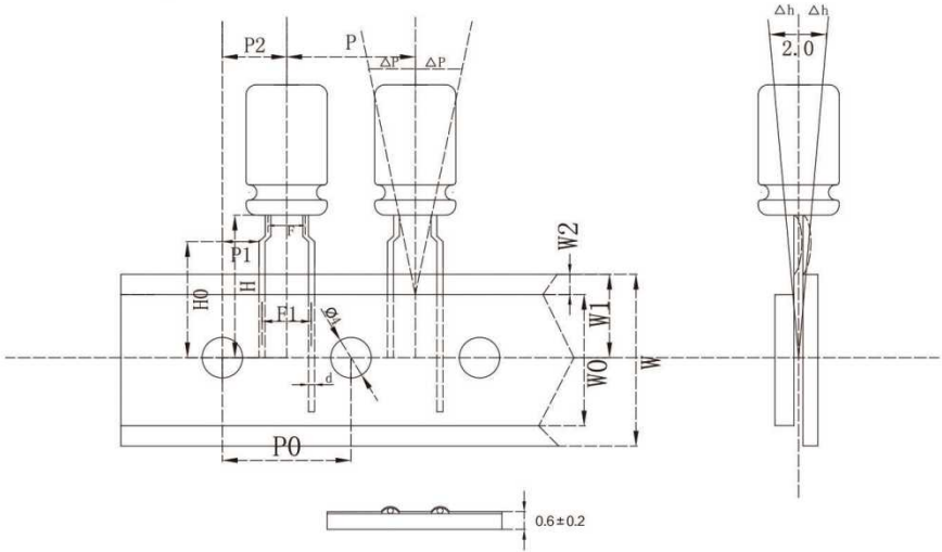
Braided tape external dimensions diagram A
